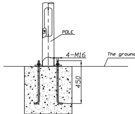
Typical concrete footing. Subject to engineered geo report provided by others
